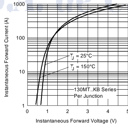
Fig. 2 - Forward Voltage Drop Characteristics
