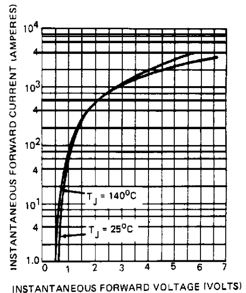
Fig. 15 - Maximum Forward Voltage Vs. Forward Current, 1N2128A Series
