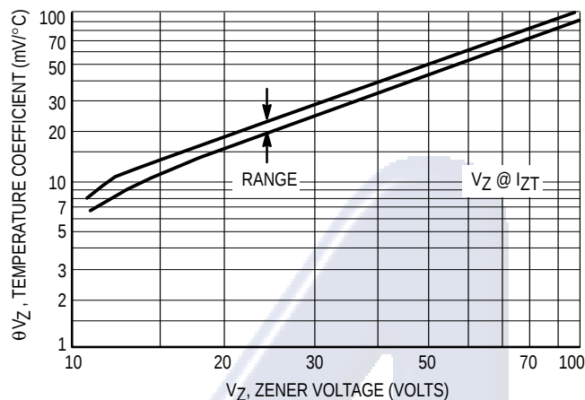
Figure 2. Temperature Coefficients
