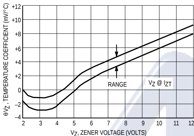
Figure 2. Temperature Coefficients
