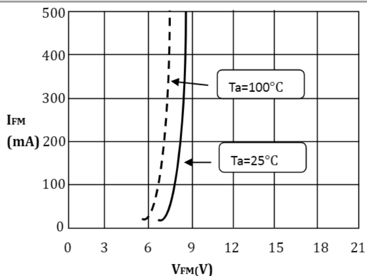
Forward Characteristics
