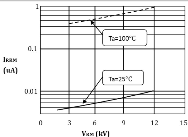
Reverse Characteristics
