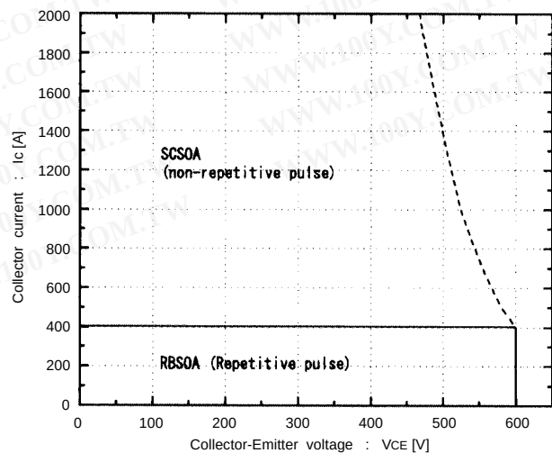
Reversed biased safe operating area +V_{GE}=15V , -V_{GE} \leq 15V , T_J \leq 125^\circ C , R_G \geq 9.1 ohm
