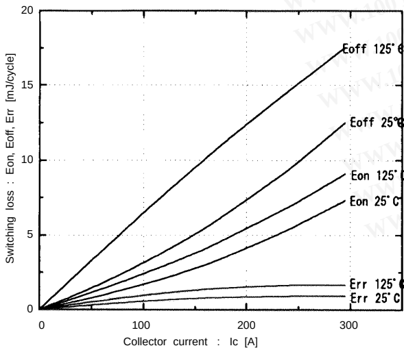
Switching loss vs. Collector current V_{CC}=300V , R_G=9.1 ohm, V_{GE}=\pm 15V
