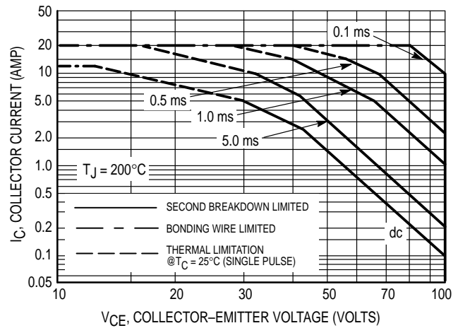
Figure 6. 2N6052, 2N6059
