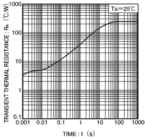
Fig.10 Transient thermal resistance (2SB1132)
