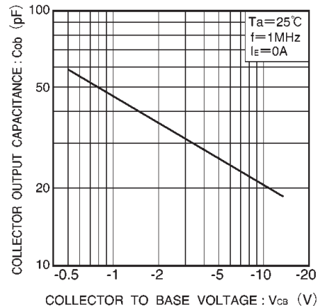
Fig.8 Collector output capacitance vs. collector-base voltage
