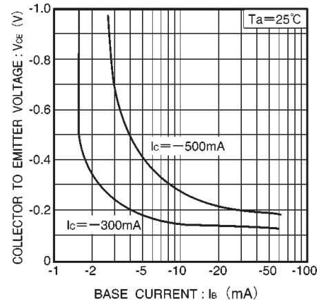
Fig.6 Collector-emitter saturation voltage vs. base current
