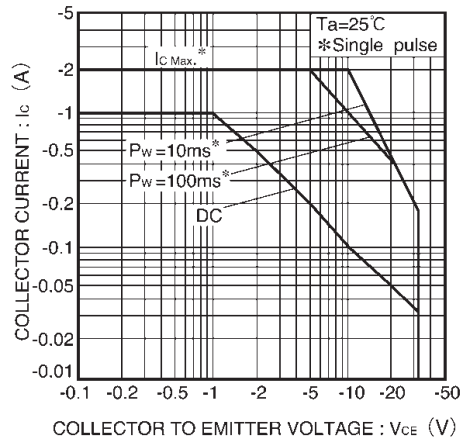
Fig.11 Safe operation area (2SB1237)
