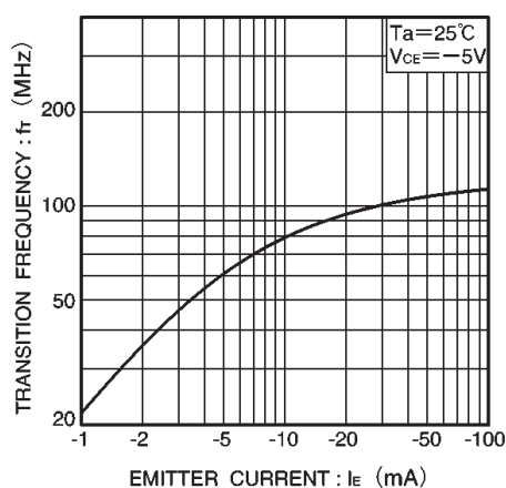
Fig.7 Gain bandwidth product vs. emitter current
