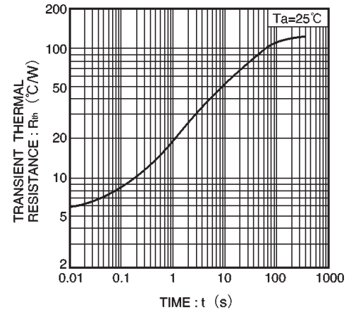
Fig.12 Transient thermal resistance (2SB1237)
