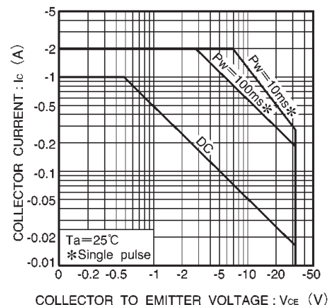
Fig.9 Safe operation area (2SB1132)
