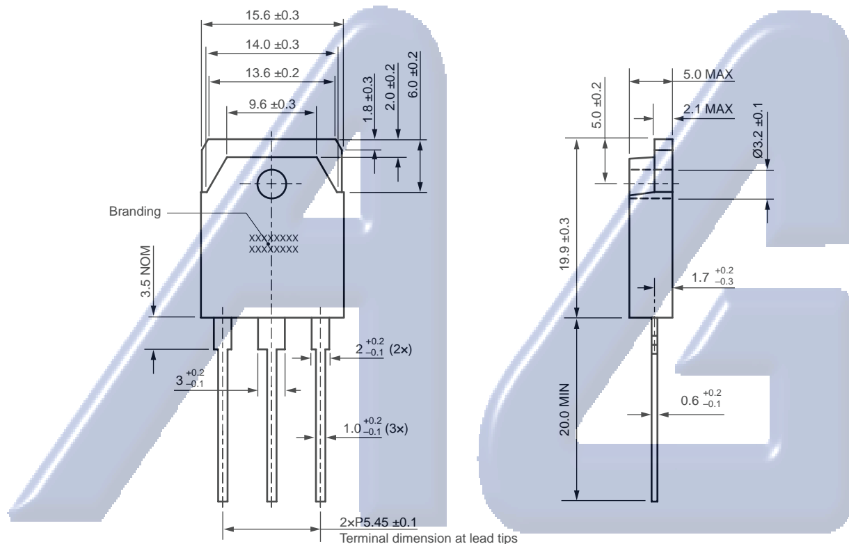
PACKAGE OUTLINE DRAWING, TO-3P
