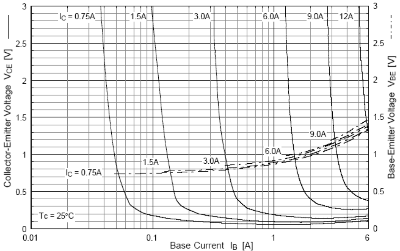
V_{CE}(\text{sat}) - I_B & V_{BE}(\text{sat}) - I_B Characteristics
