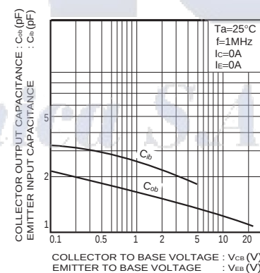
Fig.8 Capacitance vs. voltage
