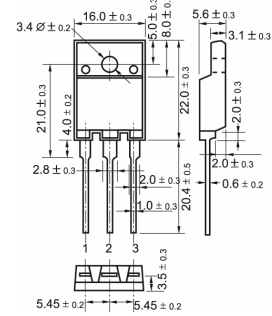
TO-3PML
