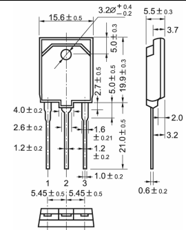
TO-3PFM
