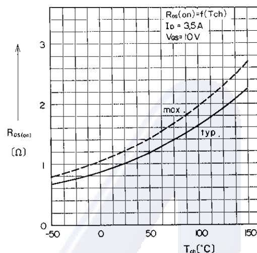
On State Resistance vs. T_{ch}
