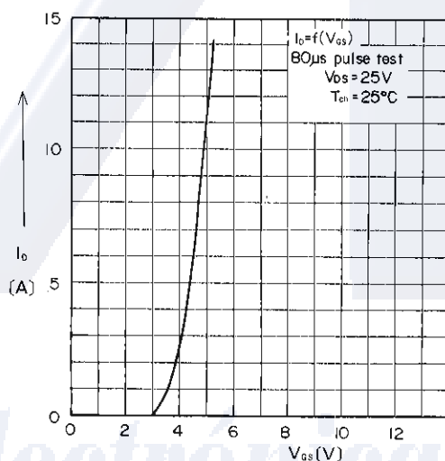
Typical Transfer Characteristic
