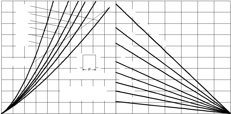
Fig. 3 - Forward Power Loss Characteristics
