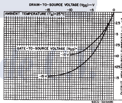
Fig. 10 - Typical p-channel output high (source) current characteristics.
