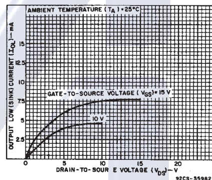
Fig. 9 - Minimum n-channel output low (sink) current characteristics.
