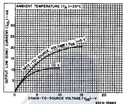
Fig. 8 - Typical n-channel output low (sink) current characteristics.
