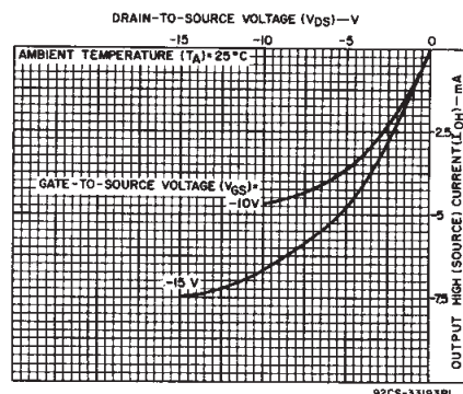
Fig. 13 - Minimum p-channel output high (source) current characteristics.
