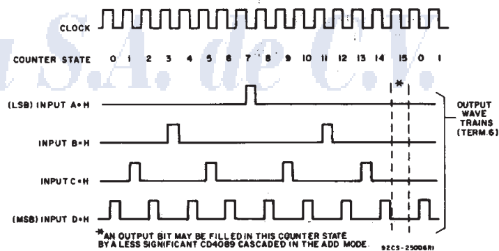
Fig. 15 – Timing diagram.
