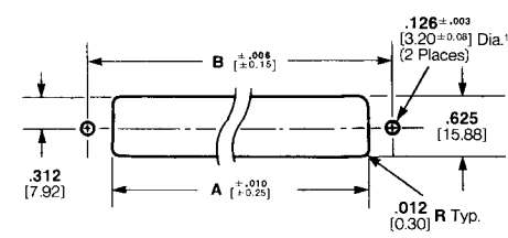
Panel Cutout Dimensions (Rear Panel Mount)
