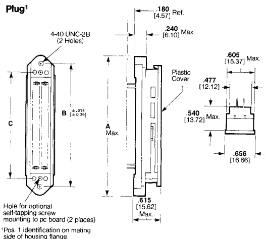
Plug 1
