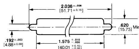
Panel Cutout for 24-Position IEEE-488 Metric
