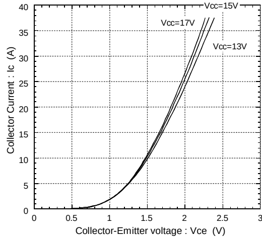
Collector current vs. Collector-Emittter voltage T_j=25^{\circ}\text{C}
