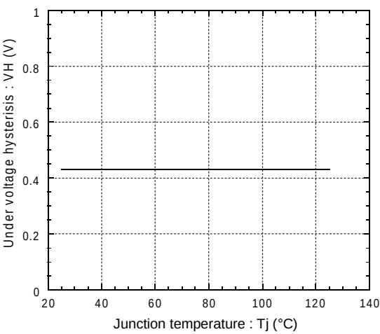
Under voltage hysteresis vs. Jnction temperature
