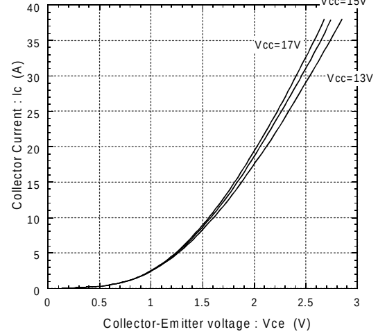
Collector current vs. Collector-Emittter voltage T_j=125^{\circ}\text{C}
