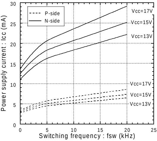
Power supply current vs. Switching frequency Tj=100°C
