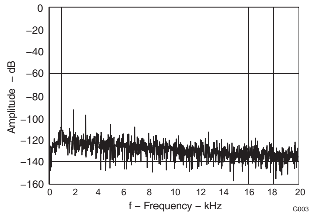
Figure 6. DAC to Line Output FFT Plot
