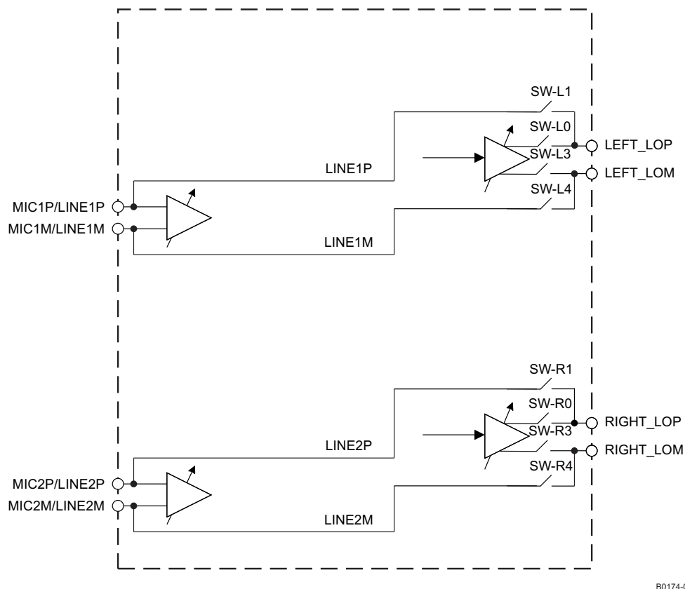
Figure 26. Passive Analog Bypass Mode Configuration
