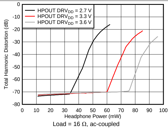
Figure 5. THD vs Headphone Power, 16-Ω Load
