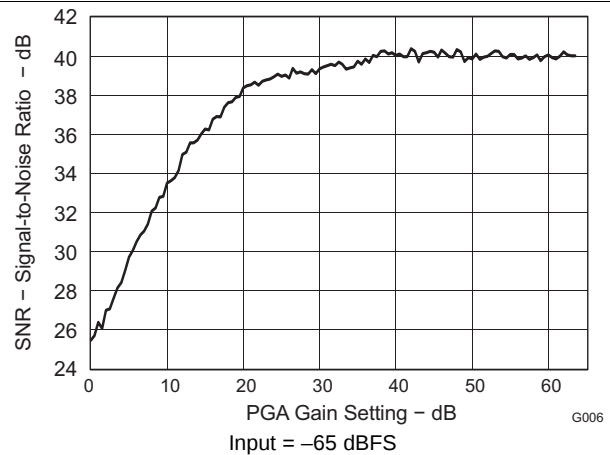
Figure 8. ADC SNR vs PGA Gain Setting, -65-dBFS Input
