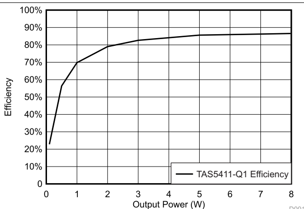
Figure 189. Efficiency Curve for the TAS5411-Q1
