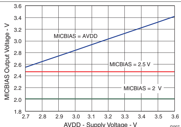
Figure 190. MICBIAS Output Voltage vs AVDD for the TLV320AIC3109-Q1
