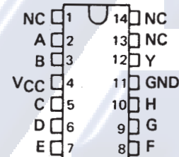
SN5430 . . . W PACKAGE (TOP VIEW)
