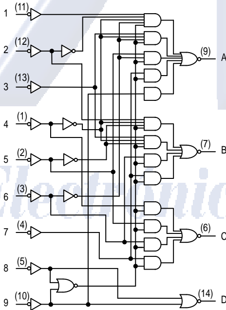
SN54/74LS147
