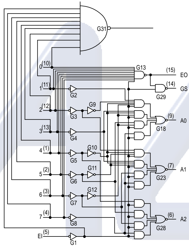
SN54/74LS748
