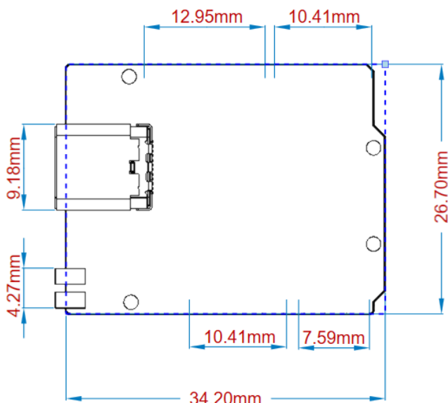
Board outline
