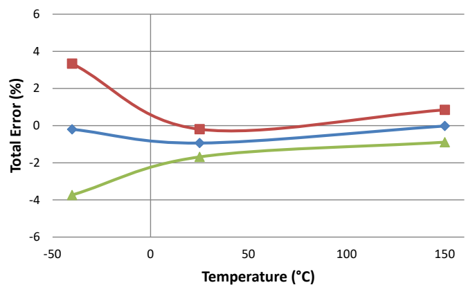
Total Error at I_{PR(max)} vs. Temperature
