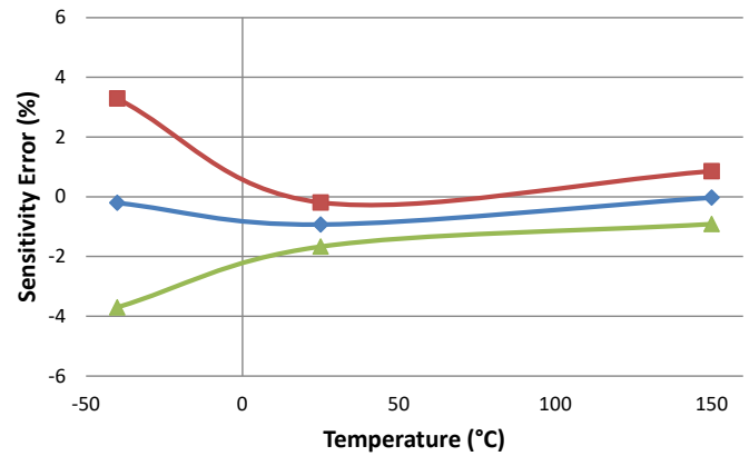
Sensitivity Error vs. Temperature
