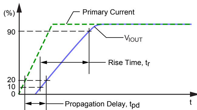
Figure 7: Rise Time ( t_r ) and Propagation Delay ( t_{pd} )
