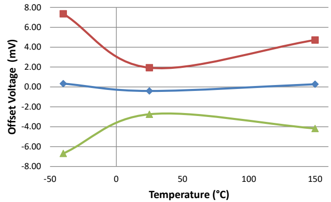
Offset Voltage vs. Temperature
