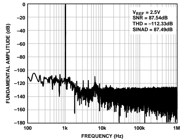
Figure 15. 1 kHz, -0.5 dBFS Input Tone FFT, Wide View, V_{REF} = 2.5V
