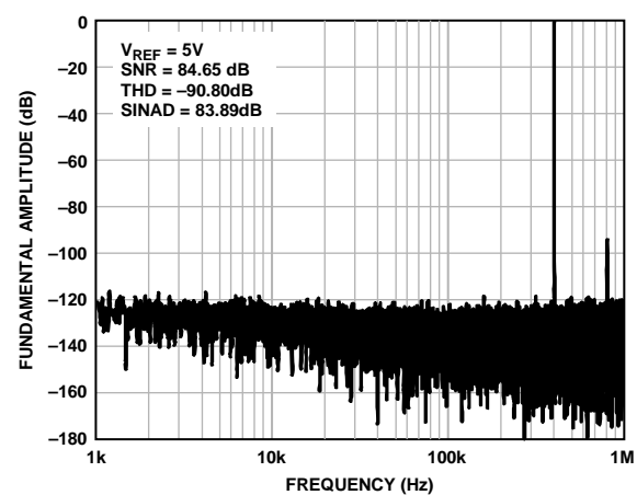
Figure 16. 400 kHz, -0.5 dBFS Input Tone FFT, Wide View
