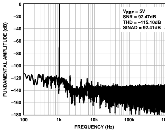
Figure 12. 1 kHz, -0.5 dBFS Input Tone Fast Fourier Transform (FFT), Wide View, V_{REF} = 5V
