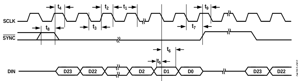
Figure 2. AD5060 Timing Diagram
