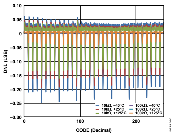
Figure 10. DNL vs. Code (AD5143)
