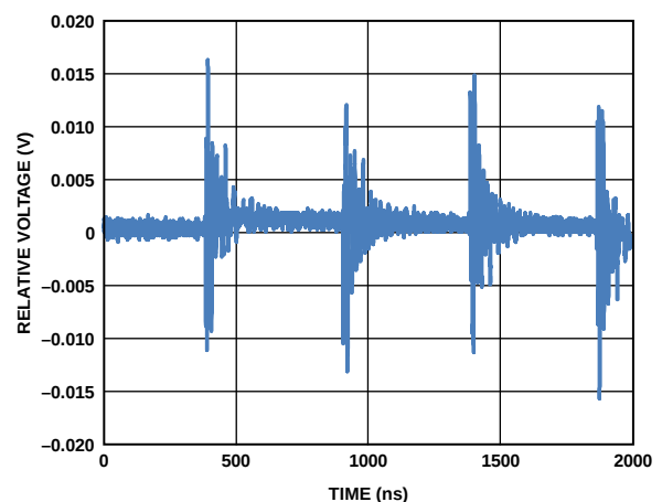
Figure 28. Digital Feedthrough
