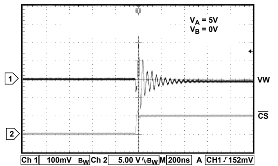
Figure 25. Digital Feedthrough
