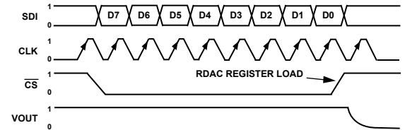
Figure 37. SPI Interface Timing Diagram ( V_A = 5\text{ V} , V_B = 0\text{ V} , V_W = V_{OUT} )
