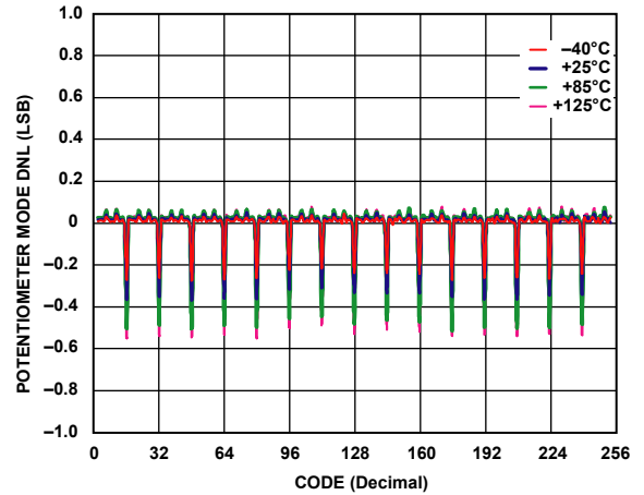
Figure 7. DNL vs. Code, V_{DD} = 5\text{ V}
