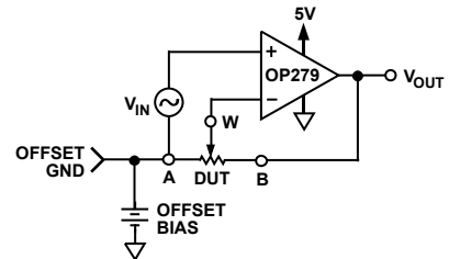
Figure 33. Test Circuit for Noninverting Gain
