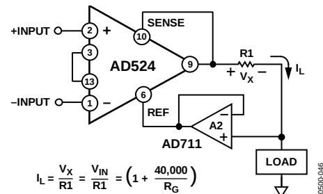
Figure 46. Voltage-to-Current Converter
