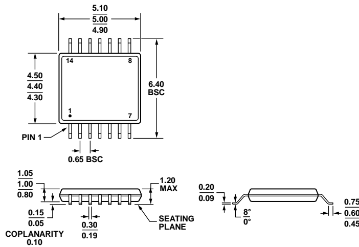
COMPLIANT TO JEDEC STANDARDS MO-153-AB-1 Figure 76. 14-Lead Thin Shrink Small Outline Package [TSSOP] (RU-14) Dimensions shown in millimeters
