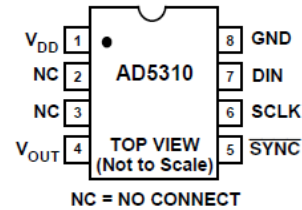
NC = NO CONNECT Figure 4. μSOIC
