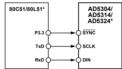
Figure 38. AD5304/AD5314/AD5324 to 80C51/80L51 Interface
