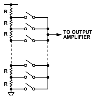
Figure 31. Resistor String
