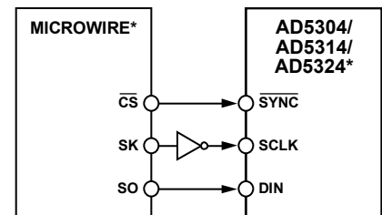
Figure 39. AD5304/AD5314/AD5324 to MICROWIRE Interface
