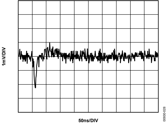
Figure 26. DAC-to-DAC Crosstalk
