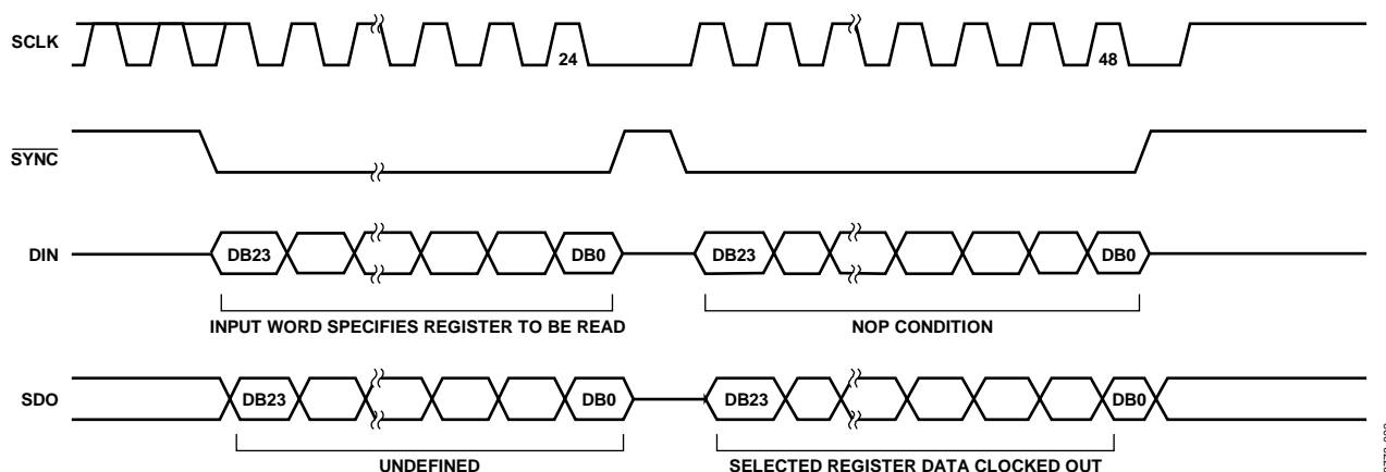
Figure 32. Readback Operation
