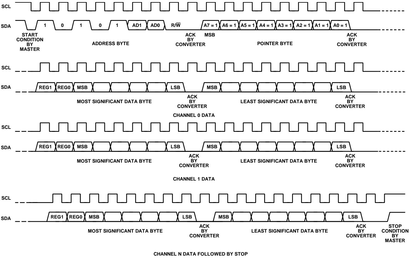
Figure 36. 2-Byte Mode I 2 C Write Operation
