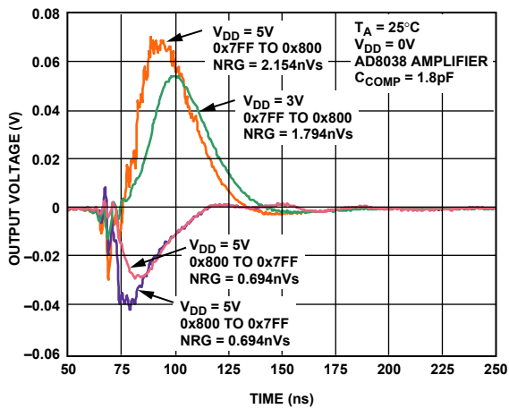
Figure 30. Midscale Transition, V_{REF} = 0\text{V}
