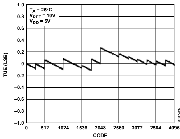
Figure 17. TUE vs. Code (12-Bit DAC)
