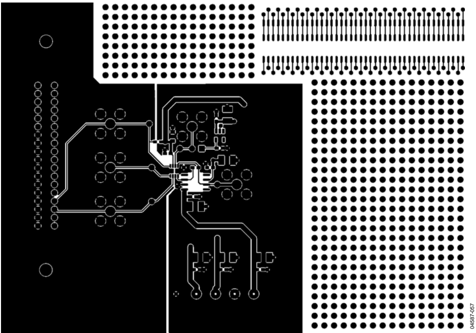
Figure 62. Component-Side Artwork
