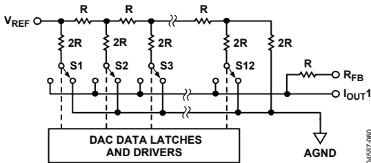
Figure 42. AD5452 Simplified Ladder
