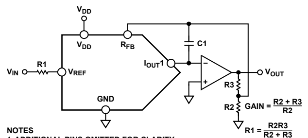
Figure 47. Increasing Gain of Current-Output DAC
