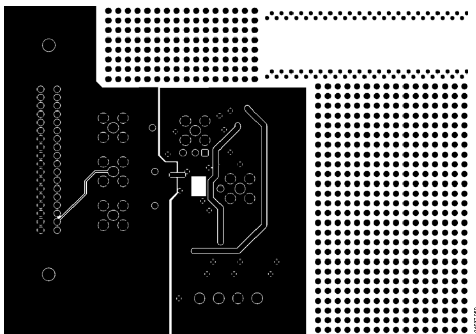
Figure 64. Solder-Side Artwork
