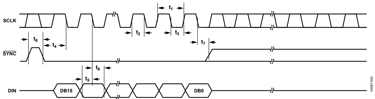
Figure 2. Timing Diagram
