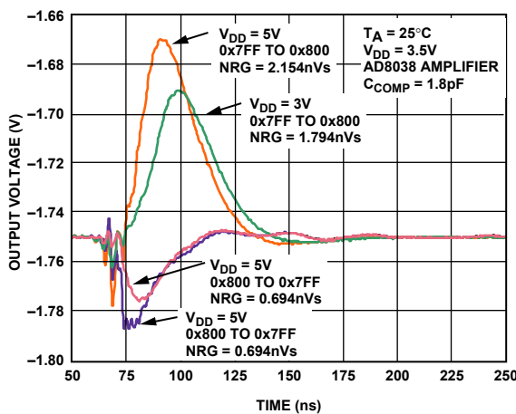
Figure 31. Midscale Transition, V_{REF} = 3.5\text{V}
