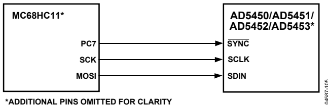
Figure 58. MC68HC11-to-AD5450/AD5451/AD5452/AD5453 Interface
