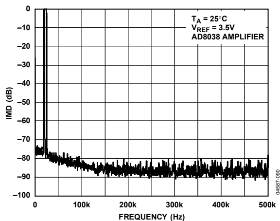
Figure 40. Wideband IMD, f_{OUT} = 20\text{ kHz} , 25\text{ kHz} , Clock = 1\text{ MHz}
