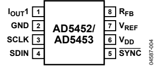
Figure 4. MSOP Pin Configuration
