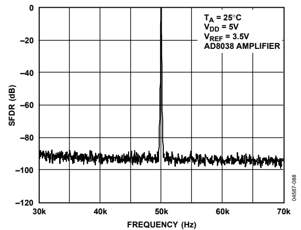
Figure 38. Narrow-Band SFDR, f_{OUT} = 50\text{ kHz} , Clock = 1 MHz
