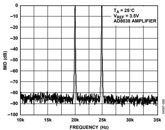
Figure 39. Narrow-Band IMD, f_{OUT} = 20\text{ kHz} , 25\text{ kHz} , Clock = 1\text{ MHz}
