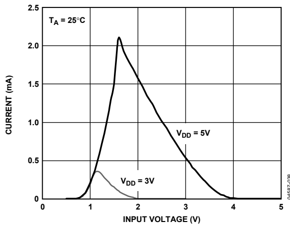
Figure 23. Supply Current vs. Logic Input Voltage
