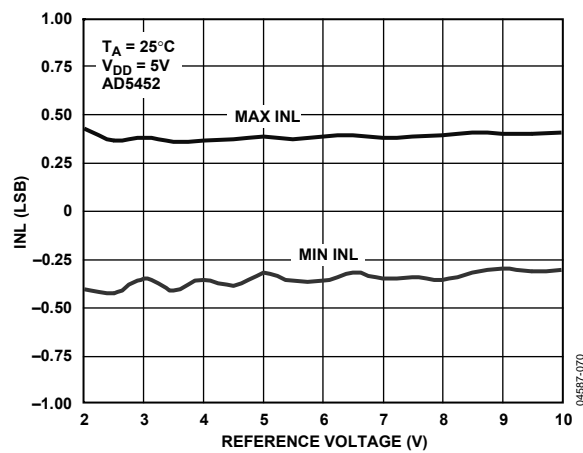
Figure 13. INL vs. Reference Voltage
