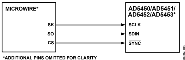
Figure 59. MICROWIRE-to-AD5450/AD5451/AD5452/AD5453 Interface
