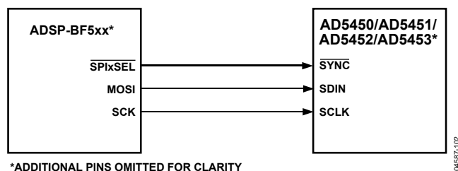
Figure 55. ADSP-BF5xx-to-AD5450/AD5451/AD5452/AD5453 Interface
