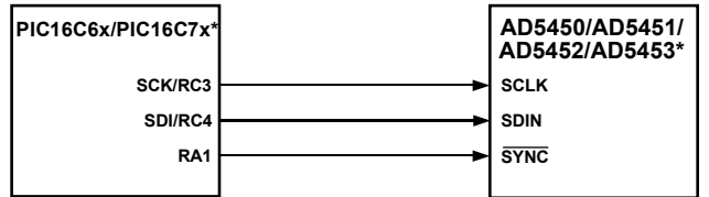
Figure 60. PIC16C6x/7x-to-AD5450/AD5451/AD5452/AD5453 Interface
