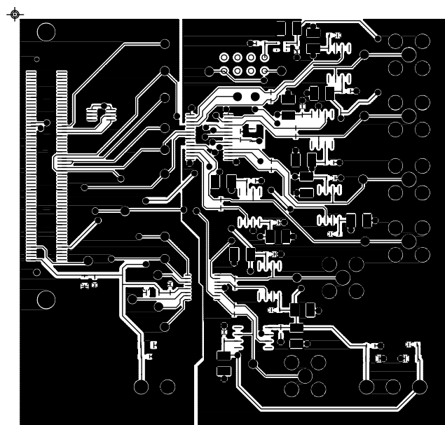
Figure 31. Component Side
