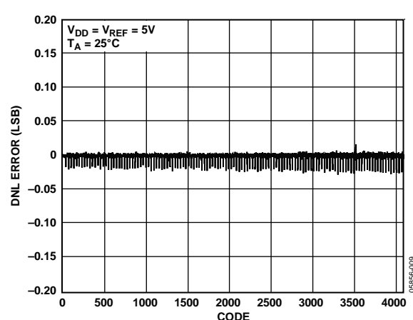
Figure 10. AD5624R DNL, External Reference
