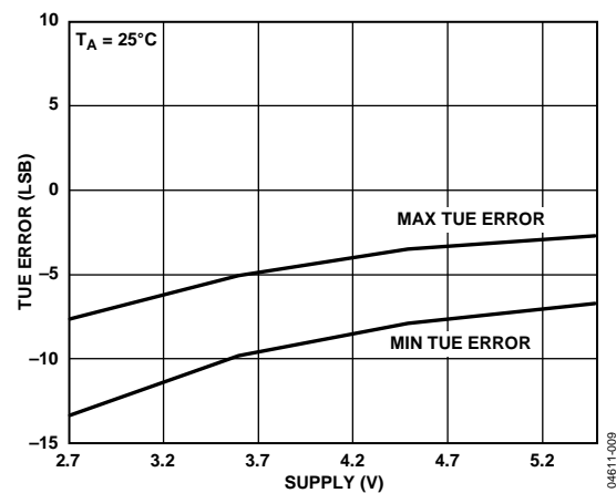
Figure 10. Total Unadjusted Error (TUE) vs. Supply at 25^\circ C
