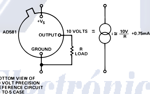
Figure 11. A Two-Component Precision Current Limiter
