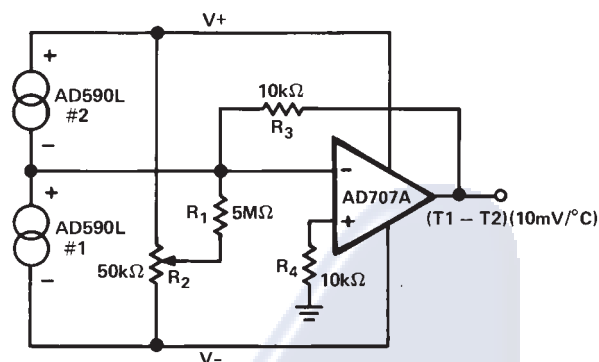
Figure 12. Differential Measurements
