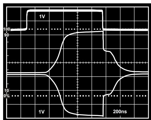
Figure 18. Gain Control Channel Response Time
