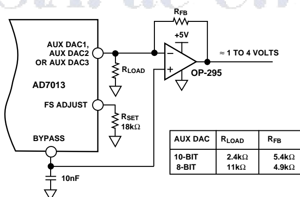
Figure 23. External Op Amp Circuitry to Extend Output Voltage Range
