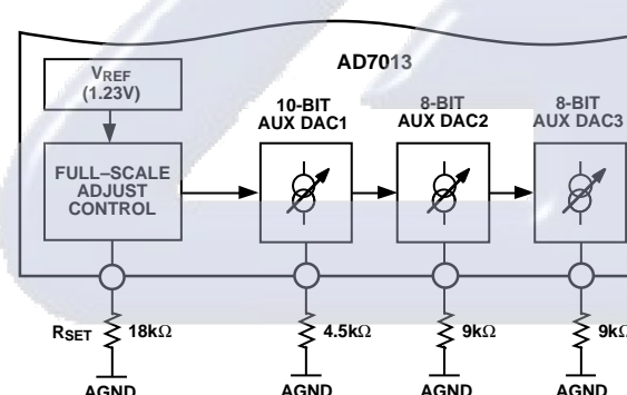
Figure 22. AUX DACs
