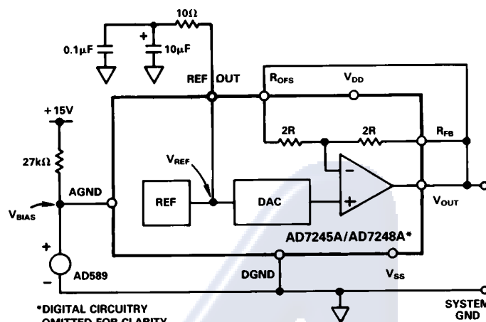
Figure 9. AGND Bias Circuit
