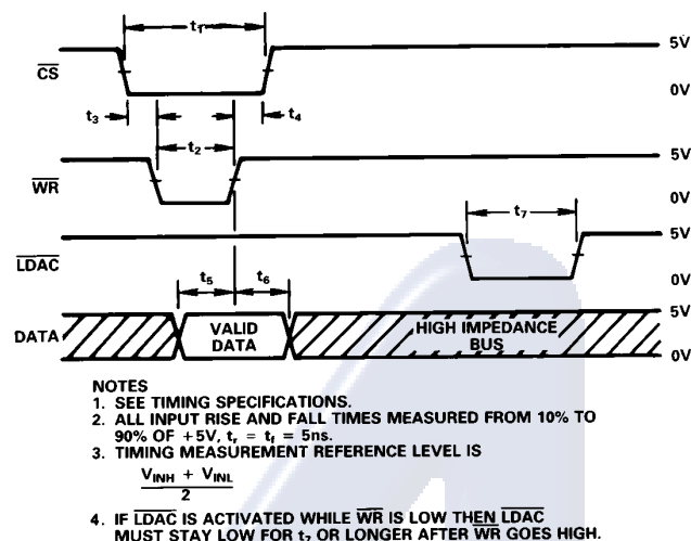
Figure 5. AD7245A Write Cycle Timing Diagram
