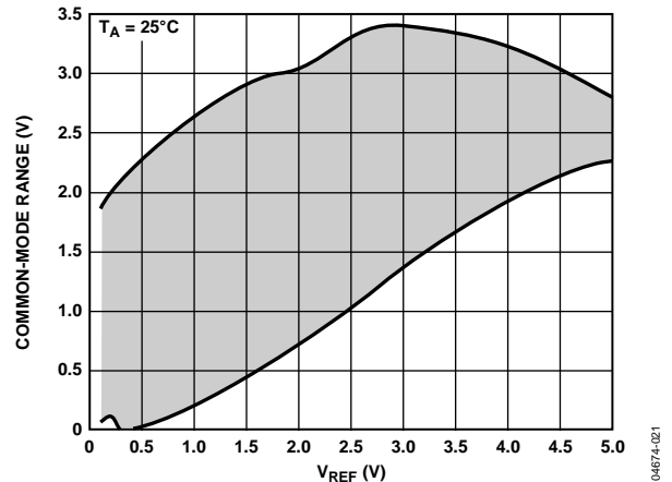
Figure 24. Input Common-Mode Range vs. V_{REF} (0 to V_{REF} Range, V_{DD} = 5 V)
