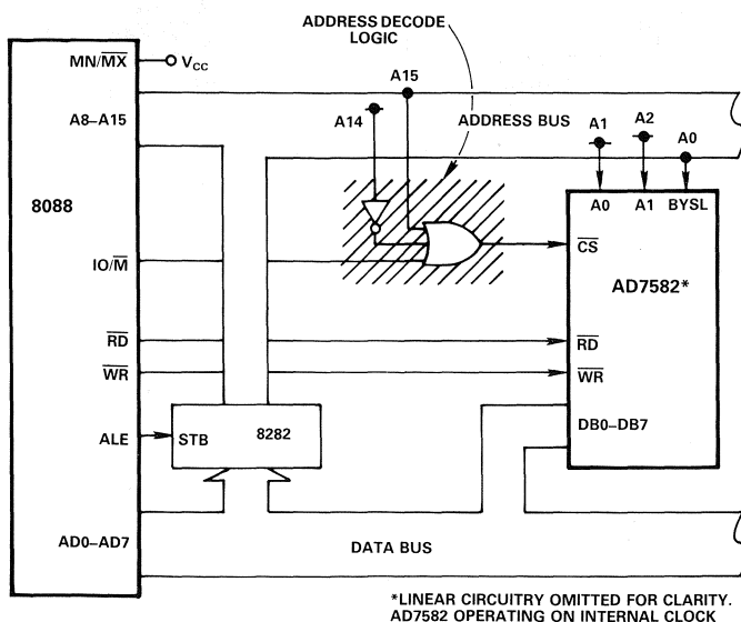
Figure 21. AD7582 – 8088 Interface
