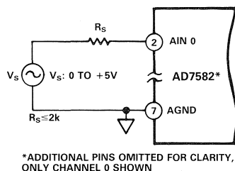
Figure 11. Unipolar 0 to +5V Operation
