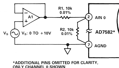
Figure 13. Unipolar 0 to +10V Operation
