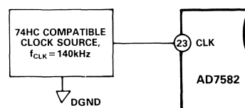
Figure 8. External Clock Operation
