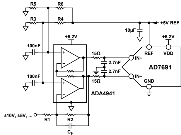
Figure 32. Single-Ended-to-Differential Driver Circuit
