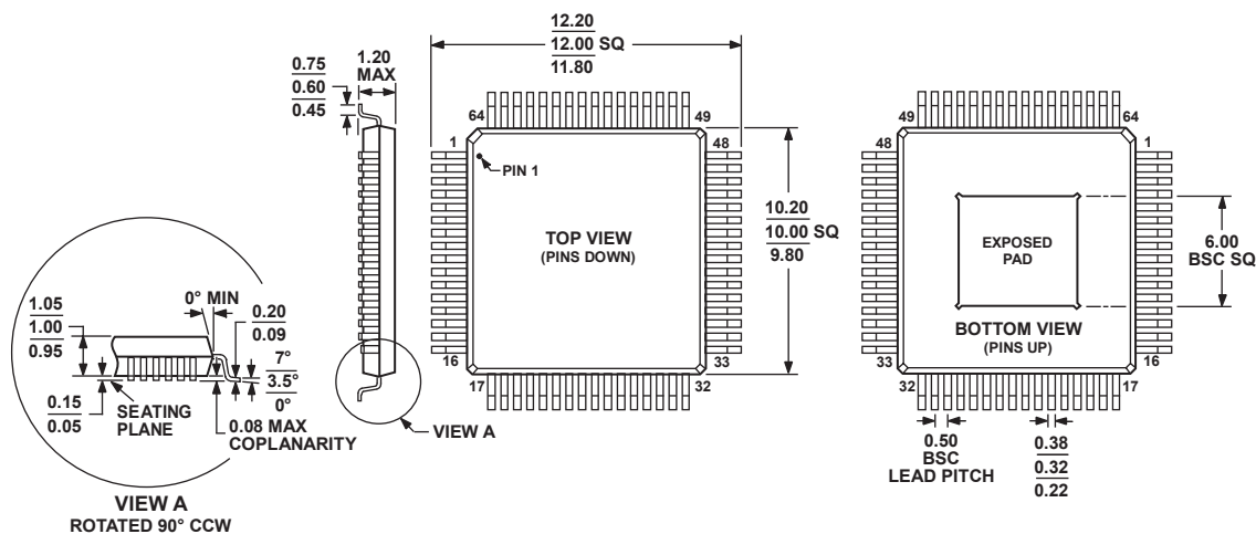
Figure 59. 64-Lead Thin Quad Flat Package, Exposed Pad [TQFP_EP] (SV-64-2) Dimensions shown in millimeters
