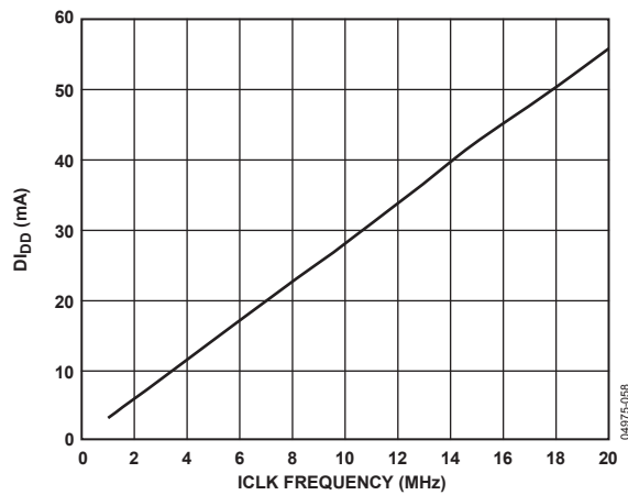
Figure 37. Decimate \times 8 , D_{I\text{DD}} vs. ICLK Frequency ( DV_{DD} = 2.5\text{ V} )
