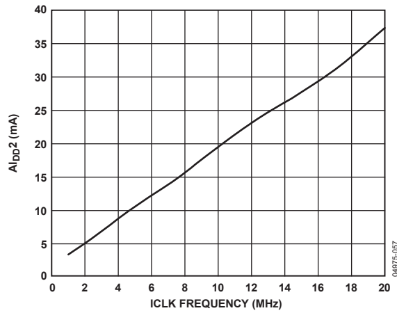
Figure 36. A_{I\text{DD}2} vs. ICLK Frequency ( AV_{DD2} = 5\text{ V} )
