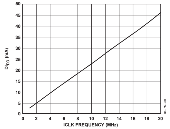
Figure 38. Decimate \times 32 , D_{I\text{DD}} vs. ICLK Frequency ( DV_{DD} = 2.5\text{ V} )
