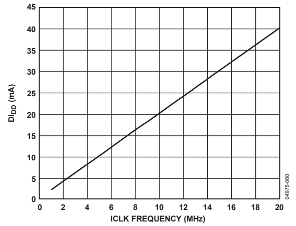
Figure 39. Decimate \times 256 , D_{I\text{DD}} vs. ICLK Frequency ( DV_{DD} = 2.5\text{ V} )
