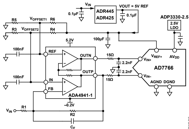
Figure 41. Driving the AD7766 from a Single-Ended Source
