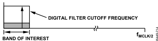
Figure 30. Digital Filter Cutoff Frequency
