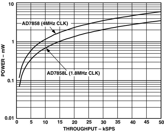
Figure 24. Power vs. Throughput Rate
