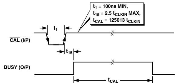
Figure 25. Timing Diagram for Full Self-Calibration
