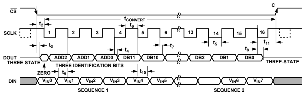
Figure 29. AD7928 Writing to SHADOW Register Timing Diagram
