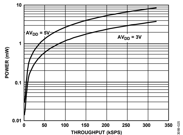
Figure 25. AD7928 Power vs. Throughput Rate
