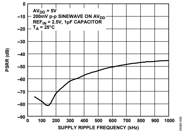
Figure 6. AD7928 PSRR vs. Supply Ripple Frequency
