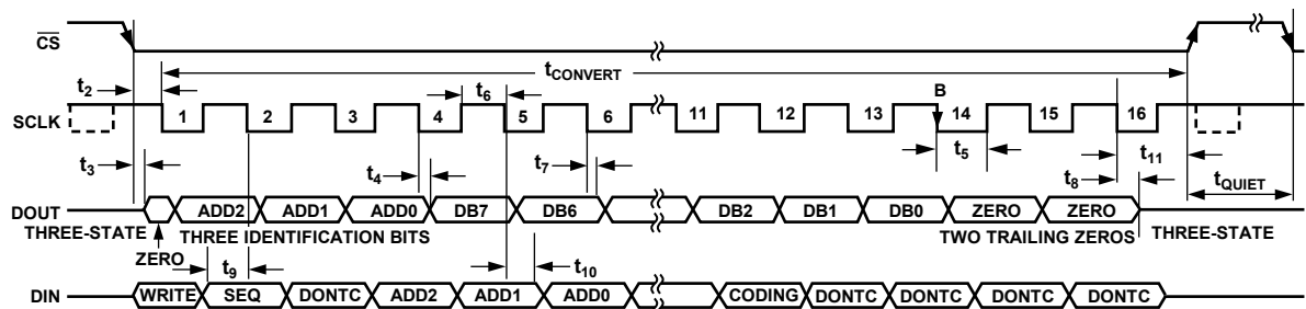
Figure 27. AD7918 Serial Interface Timing Diagram
