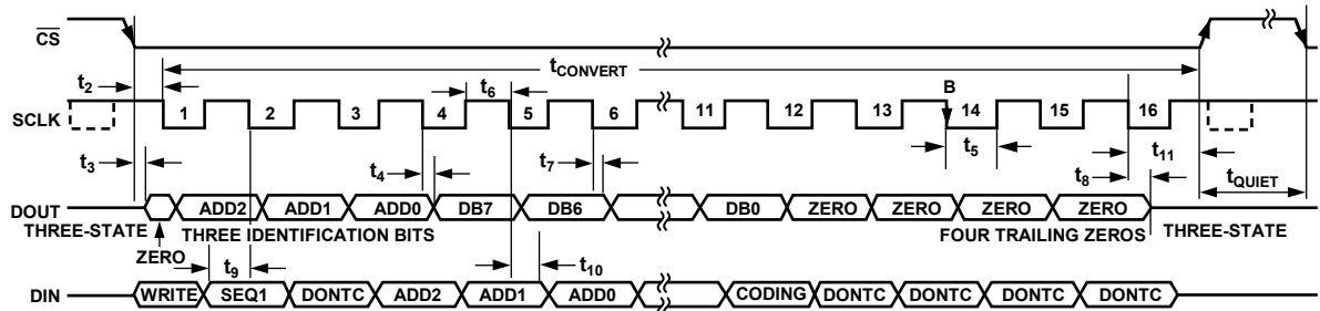
Figure 26. AD7908 Serial Interface Timing Diagram
