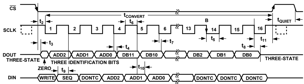
Figure 28. AD7928 Serial Interface Timing Diagram
