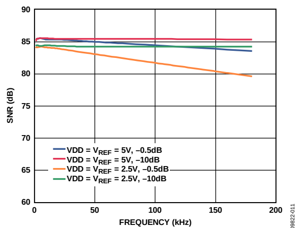
Figure 11. SNR vs. Frequency
